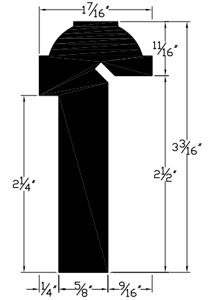
Exterior T-Astragal for 2-1/4" Door
