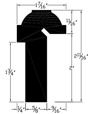
Exterior T-Astragal for 1-3/4" Door
