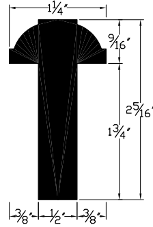
Interior T-Astragal for 1-3/4" Door
