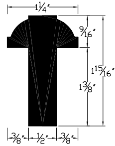
Interior T-Astragal for 1-3/8" Door
